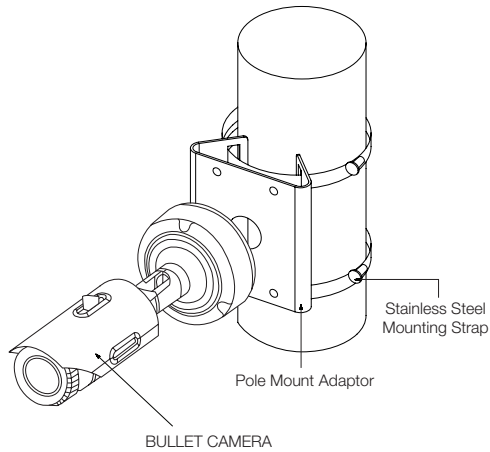
BULLET CAMERA
